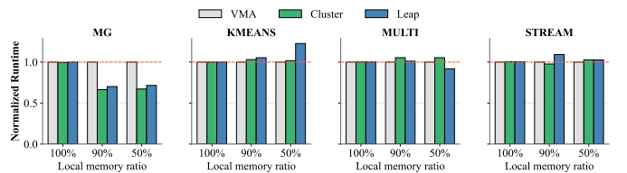
Fig. 3: Performance comparison of prefetching strategies across different applications under varying memory ratios. (i.e., the local memory ratio drops from 0.9 to 0.5), the OS tries to evict a larger volume of active pages to far memory.
