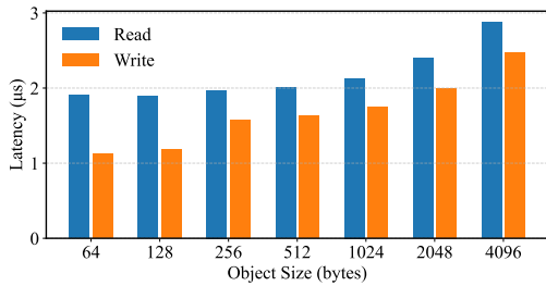
Fig. 1: Read/Write latencies of different objects via One-Sided RDMA ( \mu\text{s} ).
