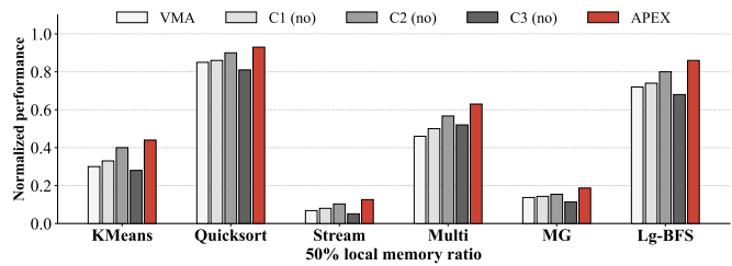
Fig. 9: Normalized ablation performance.
