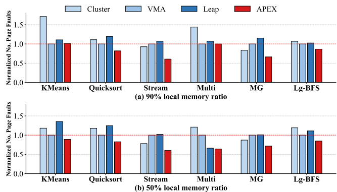
Fig. 10: Normalized number of major page faults (VMA-based). A larger value indicates a higher frequency of major page faults, whereas a smaller value indicates a lower frequency.
