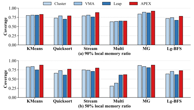
Fig. 12: Coverage of prefetching strategies under different local memory ratio.
